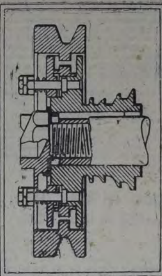
Fig. 2. — Damper-desbrague, tipo Lancheater
